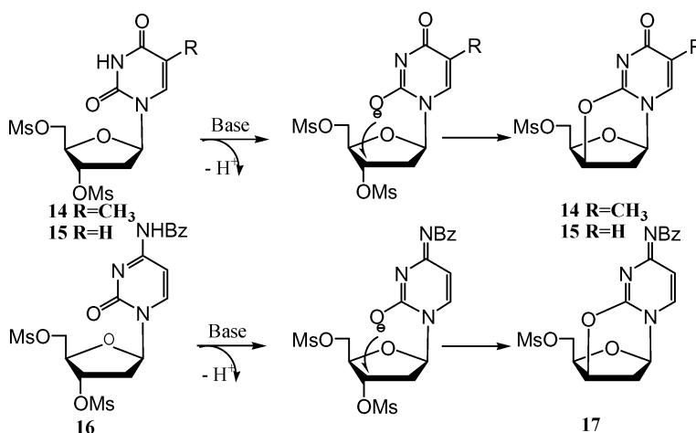
FIGURE 1 The differences between 2'-deoxy-uridine and cytosine in the process of forming 2,3'-anhydronucleosides.
