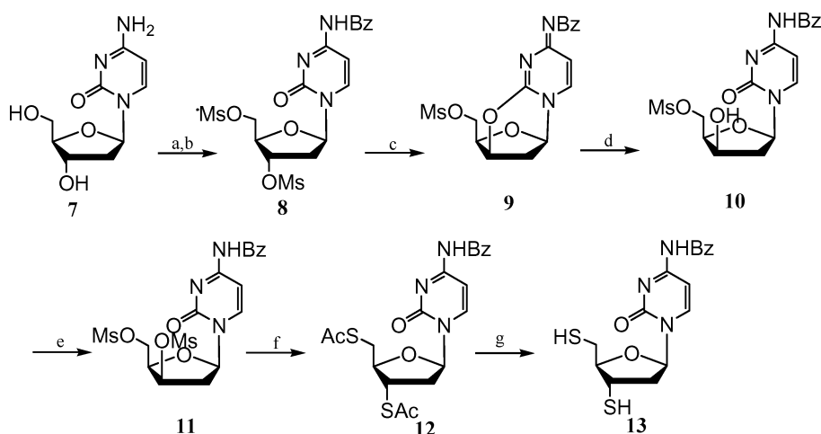
SCHEME 2 Synthetic route for 4-benzoyl-3',5'-dithio-2'-deoxycytidine. a) 1) Me 3 SiCl, pyridine, BzCl; 2) H 2 O, NH 3 ·H 2 O, 96%; b) MsCl, pyridine, 92%; c) DBU, CH 3 CN, 87%; d) Dowex, 1×2, OH ion exchange resin, EtOH/H 2 O, 75%; e) MsCl, pyridine, 91%; f) KSac, DMF, N 2 , 70%; g) EtSNa, EtSH, N 2 , 80%.
