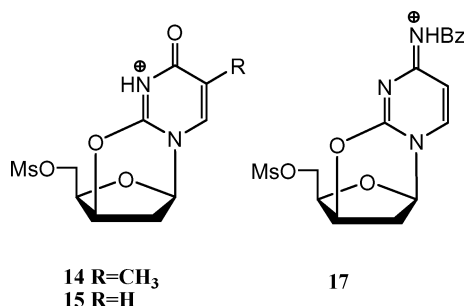
FIGURE 2 The difference between 2,3'-anhydronuridine and cytidine in the process of protonation.
