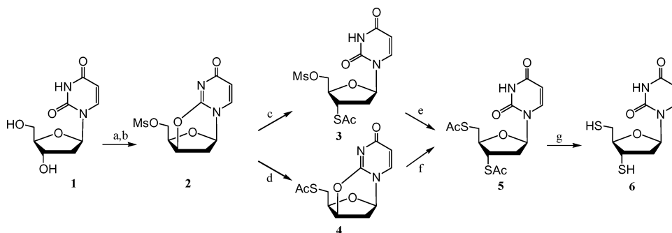
SCHEME 1 Synthetic route for 3',5'-dithio-2'-deoxyuridine. a) MsCl, pyridine, 97%; b) Et 3 N, EtOH, 92%; c) AcSH, reflux, N 2 , 77%; d) KSac, DMF, N 2 , 73%; e) KSac, DMF, N 2 , 70%; f) AcSH, reflux, N 2 , 76%; g) EtSNa, EtSH, 85%.
